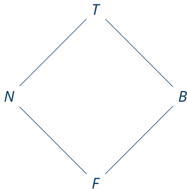
Logical Lattice (Truth Ordering)
