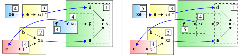
Fig. 5: Argument-based representation of the dispute states from Figure 4 (left corresponding to top, right to bottom), with similar symbols and coloring scheme. The green rectangles represent the proponent's arguments; the yellow the opponent's.
