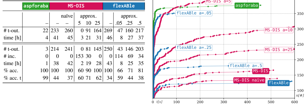
Fig. 7: Table on the left shows solving results for all 400 instances (top part) and for the 381 with known correct answers (bottom part). “–” indicates the exact solver; “naïve” denotes MS-DIS in the naïve iterative mode; “approx.” denotes approximate setup. Approximate setups compare MS-DIS with step limits 5, 10, 25 and flexABLe with opponent sampling at 5%, 25%, and 50%. Metrics: number of timeouts (#t-out.), incorrect results (#inc.), total time in hours (time [h]), accuracy excluding timeouts (% acc.), and accuracy treating timeouts as incorrect (% acc. t). All values are rounded to the nearest integer. Plot on the right shows solving times for all instances, ordered by time (x-axis: solving time in seconds, y-axis: instance index). Solid label background indicates exact solver; white background: approximate.
