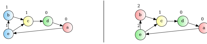
Fig. 2: Representation of two steps of a dispute for the argumentation framework \mathcal{F} = (A, R) and goal d , where A = \{a, b, c, d, e\} and R = \{(a, e), (d, a), (c, d), (b, c), (e, b), (e, c)\} . The left figure depicts the dispute state after a proponent move m(0, \mathbf{p}, d) and opponent move m(1, \mathbf{o}, c) ; the right figure depicts the state in which the proponent has won after making a m(2, \mathbf{p}, e) move. The numbers above the arguments indicate the step at which their status is determined. The status is shown via colors: green – put forward by the proponent (e.g., e at step 2 via m(2, \mathbf{p}, e) ), yellow – put forward by the opponent, red – defeated/unplayed arguments (e.g., a via defeat (0, a) ), blue – possible moves at a step (e.g., pm(1, \mathbf{p}, b) , pm(1, \mathbf{p}, e) ).
