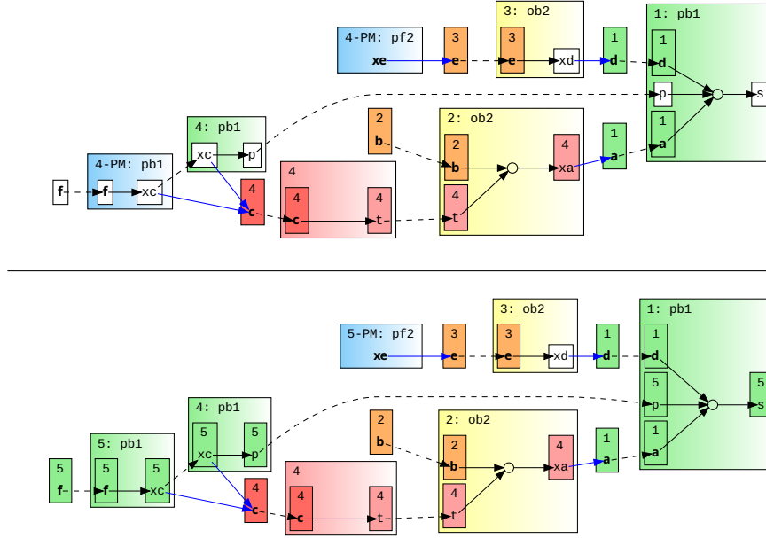
Fig. 4: Two dispute states - 4 (top) and 5 (bottom) - for the ABA framework \mathcal{F} = (\mathcal{L}, \mathcal{A}, \neg, \mathcal{R}) , where \mathcal{A} = \{a, b, c, d, e, xe\} , \neg(\tau) = \{x\tau\} for \tau \in \{a, b, c, d, e\} (there are no further contraries), and \mathcal{R} = s \leftarrow d, p, a; p \leftarrow xc; xc \leftarrow f; xd \leftarrow e; xa \leftarrow b, t; t \leftarrow c . The dispute state on the top has been obtained via the sequence of moves: m(1, \mathbf{p}, pb1, s \leftarrow p, d, a) , m(2, \mathbf{o}, ob2, xa \leftarrow b, t) , m(3, \mathbf{o}, ob2, xd \leftarrow e) , m(4, \mathbf{p}, pb1, p \leftarrow xc) . At step 4, the proponent has two possible moves: pm(4, \mathbf{p}, pf2, xe) and pm(4, \mathbf{p}, pb1, xc \leftarrow f) . Performing the latter gives rise to the move m(5, \mathbf{p}, pb1, xc \leftarrow f) and the dispute state shown at the bottom. Green pieces are introduced by the proponent, yellow ones by the opponent. Black arrows depict rules, while blue arrows represent attacks. Dashed arrows show dependencies between rules as well as between assumptions and rules. Assumptions are shown in boldface. Red rules are blocked, dark red statements are culprits and light red blocked opponents statements. Blue indicates possible moves. Numbers in squares next to a rule or assumption indicate the step at which they obtain their current status. For example, a “4” next to p \leftarrow xc indicates that this rule was introduced by the proponent at step 4, which is also when t \leftarrow c became blocked (shown in red) due to c becoming a culprit (because attacked by xc ). Additional information can be retrieved: e.g. statement s becomes a proponent’s complete piece at step 5 (indicated by the number above it), represented by comS(5, s, \mathbf{p}) ; c becomes a culprit at step 4 ( cul(4, c) ); or e and b become culprit candidates at steps 3 and 2, respectively ( culCan(3, e) and culCan(2, b) ).
