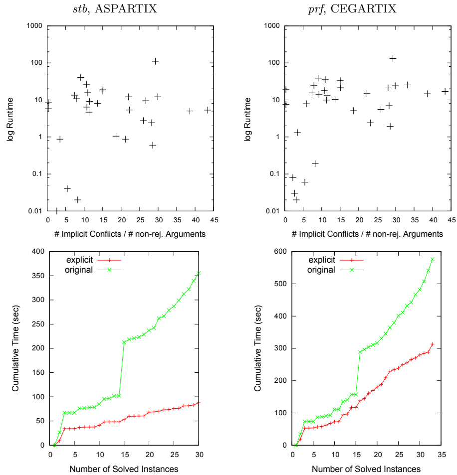
Figure A.26: Experimental results for implicit conflicts on ICCMA 2015 instances. Out of the 48 instances there are 30 (63%) for stb and 33 (69%) for prf which contain at least one implicit conflict. Among those, the number of implicit conflicts divided by the number of non-rejected arguments is 16.0 for stb and 15.6 for prf on average. The scatter plots at the top relate the number of implicit conflicts per non-rejected argument to the runtime of extension enumeration. We get a correlation coefficient of 0.16 for stb and 0.26 for prf . The diagrams at the bottom show the cumulative runtime for extension enumeration for the original set of AFS on the one hand and the corresponding explicated AFS on the other.
