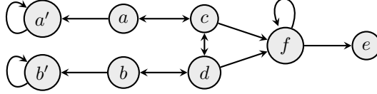
Figure 3: Argumentation framework F used in Example 1.
