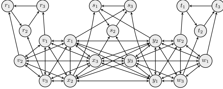
Figure 25: AF showing (\Sigma_{prf}^c \cap \Sigma_{sem}^c) \setminus (\Sigma_{stb}^c \cup \Sigma_{stg}^c) \neq \emptyset .
