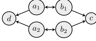
Figure C.28: AF F compactly realizing an extension-set \mathbb{S} \notin \Sigma_{adm}^c \cup \Sigma_{cf}^c under com .
