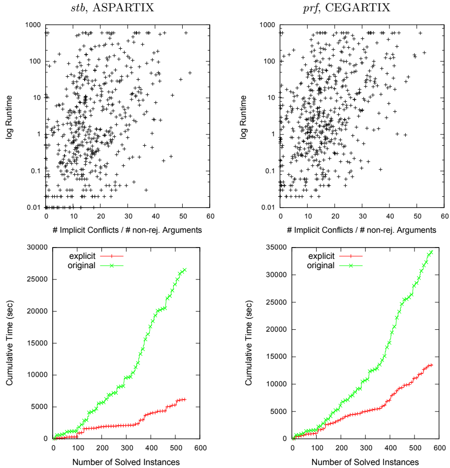
Figure A.27: Experimental results for implicit conflicts on an additional 1061 instances obtained from the same generator as the most difficult instances of ICCMA 2015. This set of AFs contains 533 (50%) for stb and 567 (53%) for prf with at least one implicit conflict. Among those, the number of implicit conflicts divided by the number of non-rejected arguments is 17.1 for stb and 17.0 for prf on average. Again, the scatter plots at the top of the figure relate the number of implicit conflicts per non-rejected argument to the runtime of extension enumeration. Now we get a correlation coefficient of 0.24 for stb and 0.30 for prf . The cumulative runtimes for extension enumeration indicating a significant speedup for the explicated AFs are shown at the bottom of the figure.
