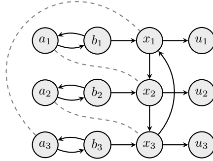
Figure 16: A non-analytic AF for prf as used in Example 6.
