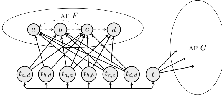
Figure 14: The AF F' from Reduction 2, for AF F = (\{a, b, c\}, \{(a, b)\}) .
