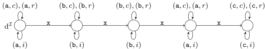
Fig. 5: An example \Sigma -friendly pointed (\mathcal{I}, d) encoding the word \text{abbac} .
