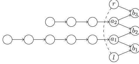
Figure 6.2: The standard (5, 3) -triple-u, where we only draw the Hasse diagram for \langle^D , and where dashed edges are \perp -edges.
