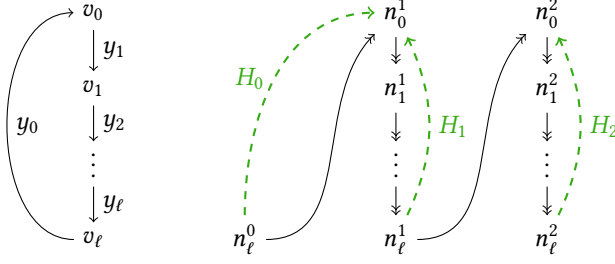
Fig. 1. Dependency cycle in LXC( \Sigma ) (left) and corresponding chain of derived nulls in chase( \Sigma, \mathcal{D} ) (right); H_0, H_1 , and H_2 denote variants of a \text{tgd} head to illustrate propagation
