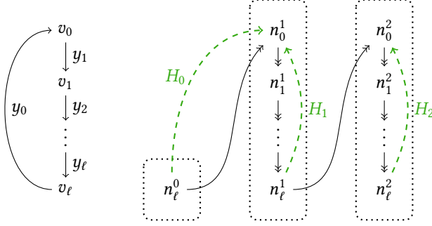
Fig. 2. Example graph LXC(\Sigma) (left) and chain of derived nulls in \text{chase}(\Sigma, \mathcal{D}) (right) from Figure 1, with nulls partitioned according to Definition 28 for the set \hat{E} = \{v_\ell \xrightarrow{y_0} v_0\}
